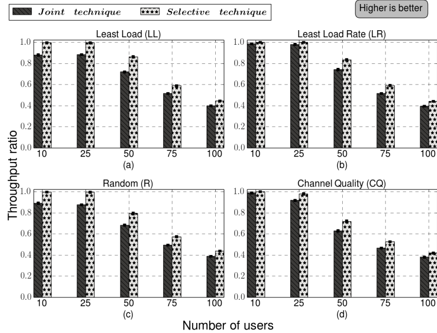
Figure 9: Throughput ratio for joint and selective techniques.
