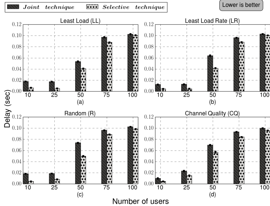
Figure 5: Delay during periodic carrier assignment operations for joint and selective techniques.
