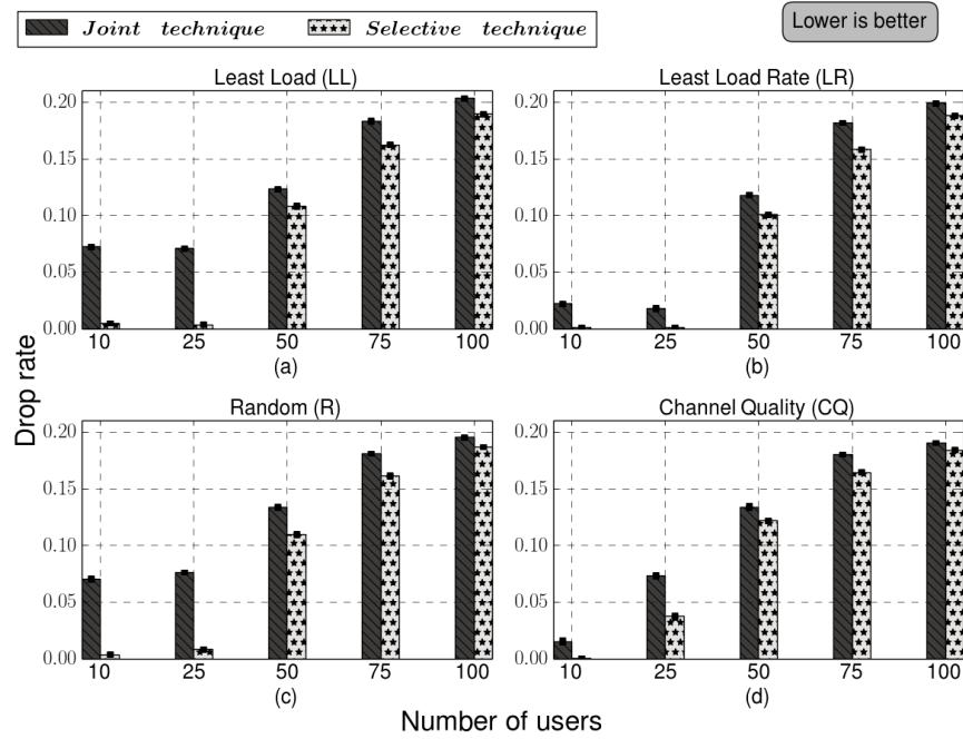
Figure 6: Packet Drop Rate during periodic carrier assignment operations for joint and selective techniques.
