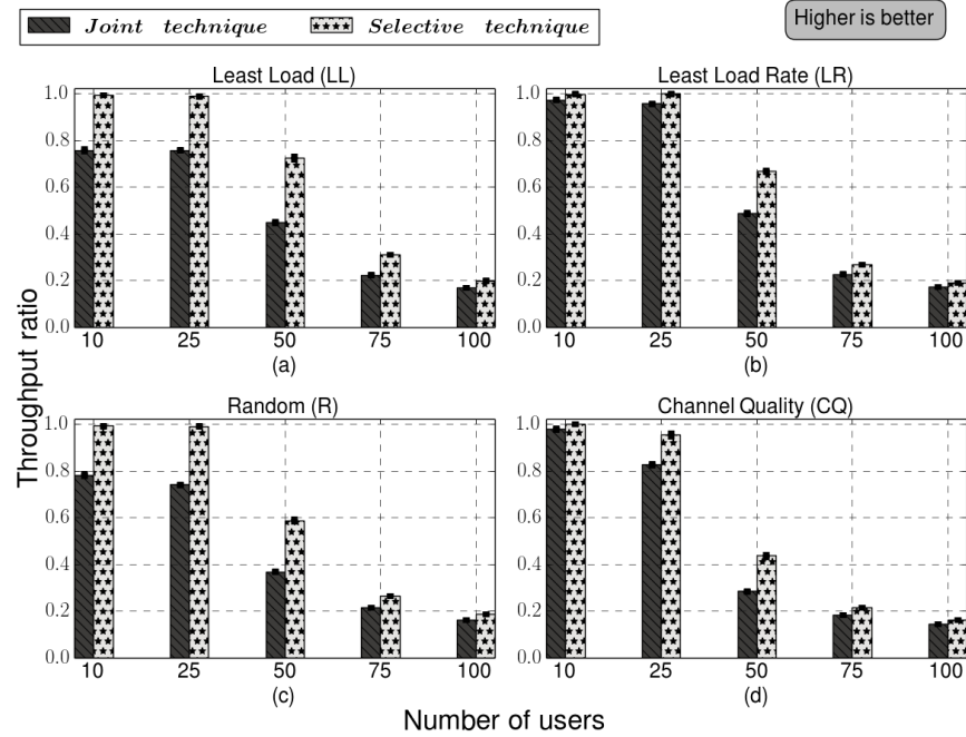
Figure 12: Throughput ratio of LTE type devices for joint and selective techniques.
