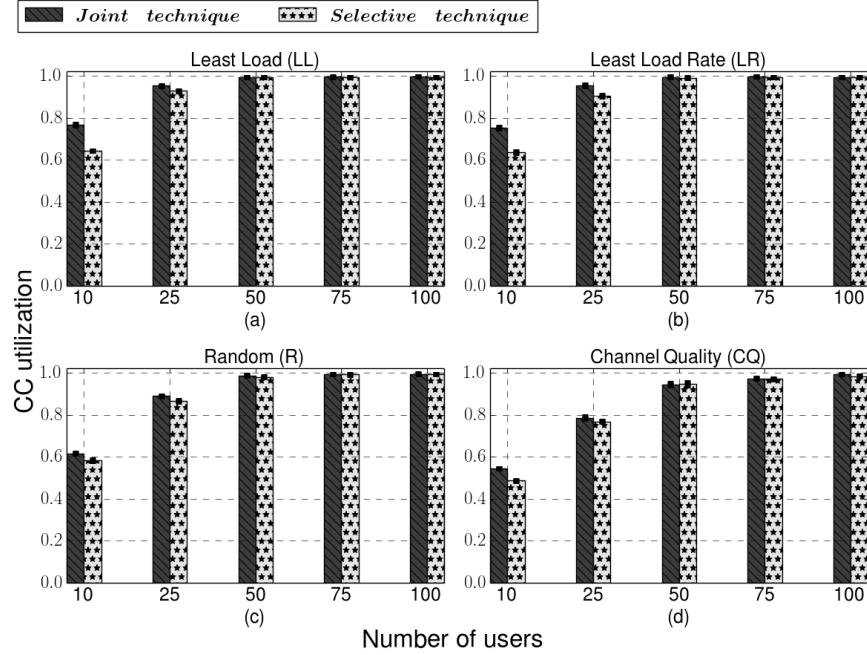
Figure 7: Utilization of CCs for joint and selective techniques.
