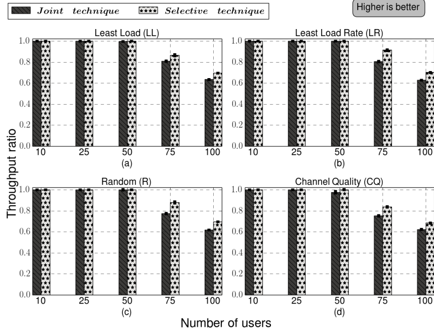
Figure 13: Throughput ratio of LTE-A type devices for joint and selective techniques.
