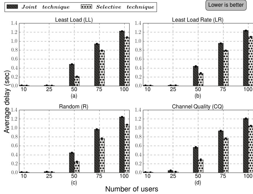
Figure 11: Average delay per packet of LTE-A type devices for joint and selective techniques.
