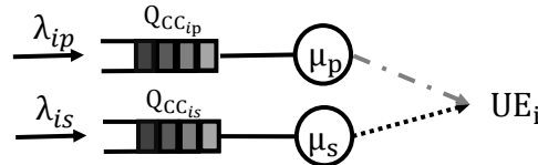
Figure 4: Downlink system model with one user with primary and secondary carrier queues.
