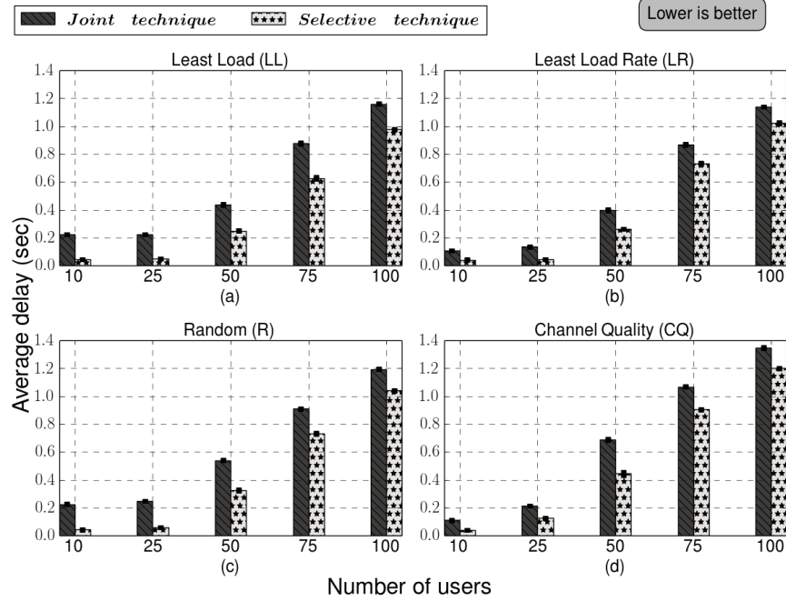
Figure 10: Average delay per packet of LTE type devices for joint and selective techniques.
