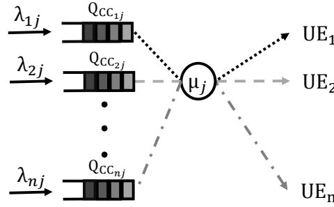
Figure 3: Downlink Disjoint Queue Model with n users and one available CC.
