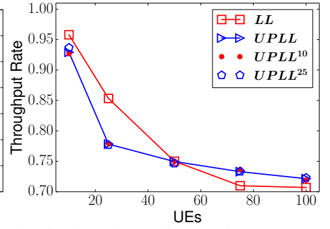
Fig. 6: Throughput of LL and UPLs by using joint assignment technique.
