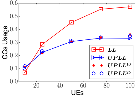
Fig. 7: CCs usage of LL and UPLs by using partial assignment technique.
